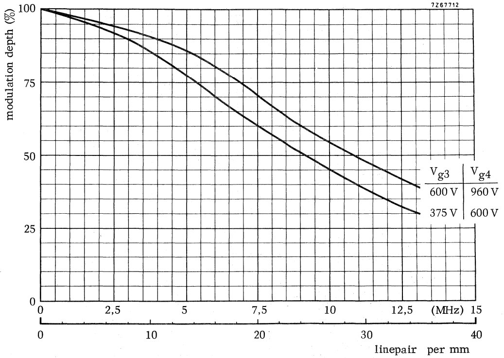
Fig. 4 Squarewave modulation transfer characteristic.
