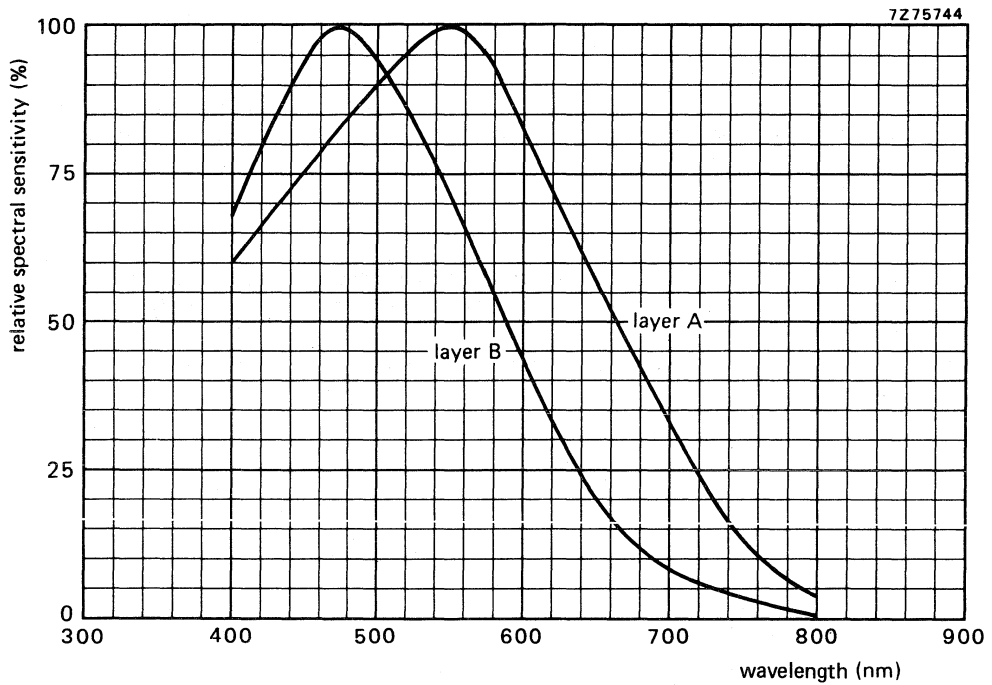
Fig. 2 Typical spectral response curves.
