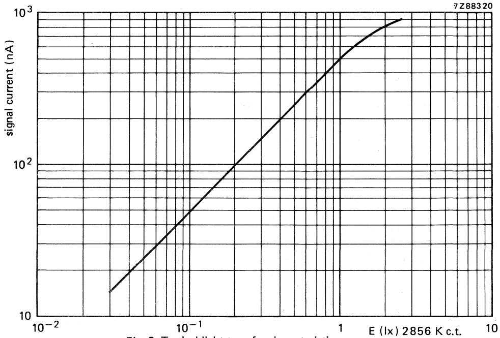
Fig. 3 Typical light transfer characteristic.
